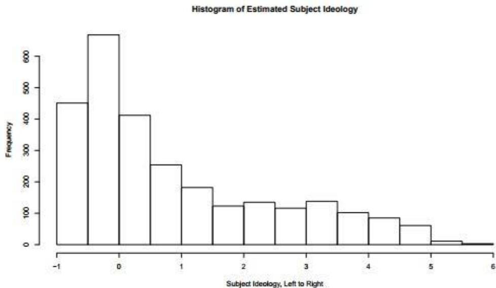
Figure 2: Ideology Distribution
